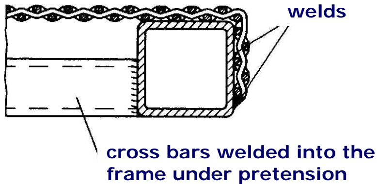
Bent wire cloth elements welded to a frame
