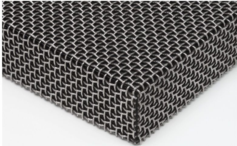
Bent wire cloth elements welded to a frame
